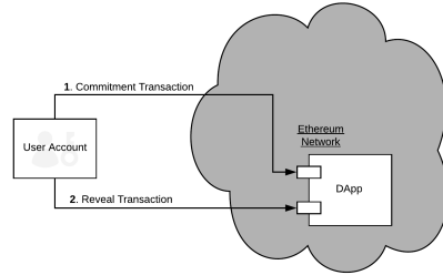
Fig. 6: Commit and Reveal. User sends a commitment transaction with the hash of the data, After the commitment period is over, user sends her reveal transaction to the DApp revealing the information that matches the commitment.
